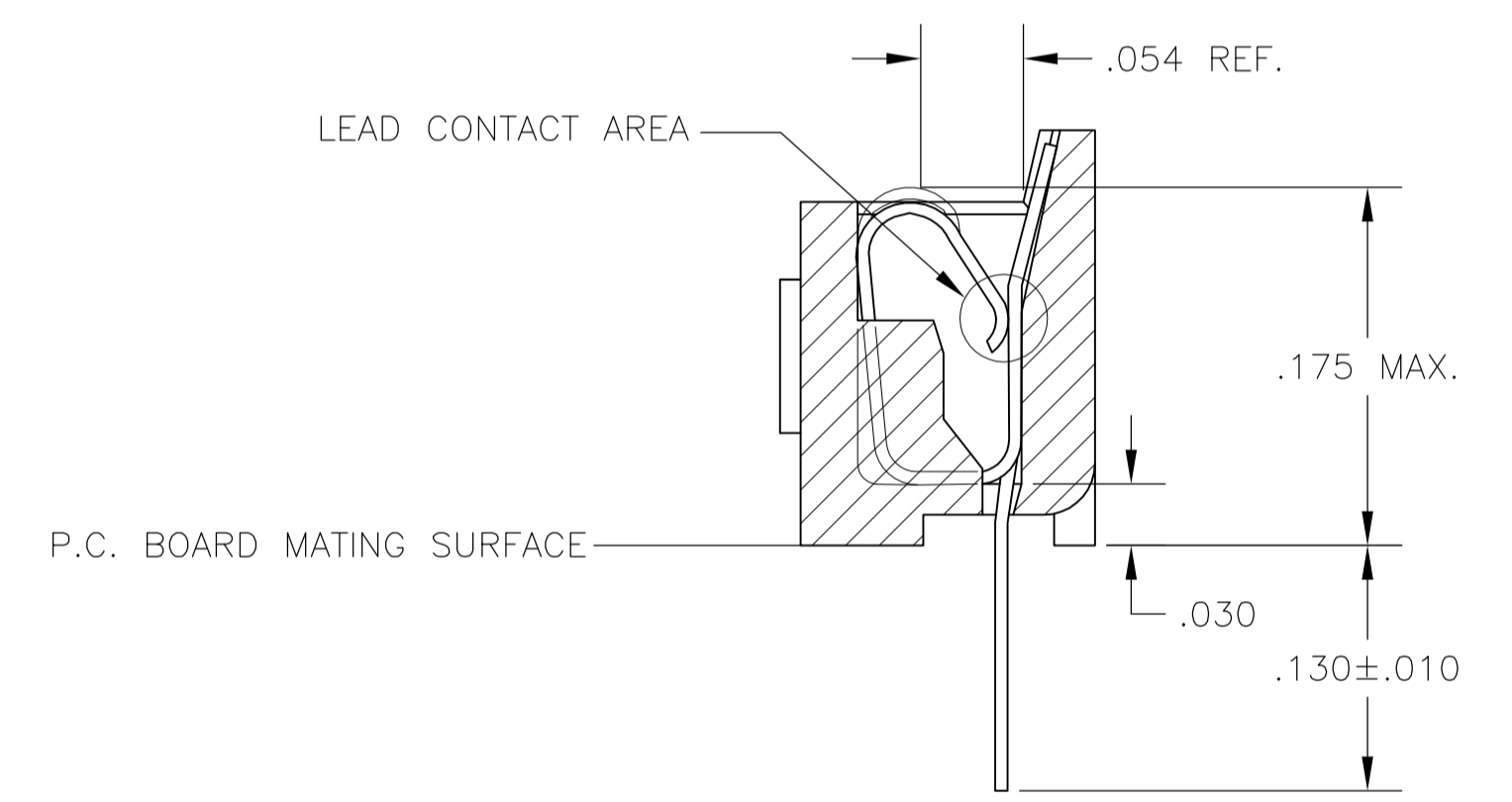
SECTION A-A ROTATED 90° CW SCALE 10:1
