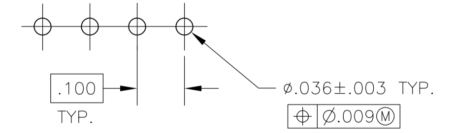
RECOMMENDED MOUNTING HOLE PATTERN
